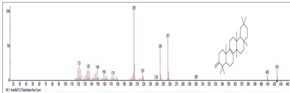
Figure 20: Mass spectrum showing presence of Friedolean-8-en-3-one (19) in Carissa congesta extract
