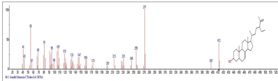
Figure 23: Mass spectrum showing presence of (3 \beta ,5 \alpha )-Stigma-7,25-dien-3-ol (22) in Carissa congesta extract
