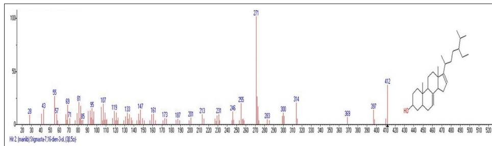
Figure 24: Mass spectrum showing presence of (3 \beta ,5 \alpha )-Stigma-7,16-dien-3-ol (23) in Carissa congesta extract
