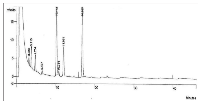
Figure 1: Gas chromatography chromatogram of garlic oil at 2 mg/ml concentration. Sample solution of garlic oil was prepared in acetone. As seen, 8 peaks are present in the chromatogram.
