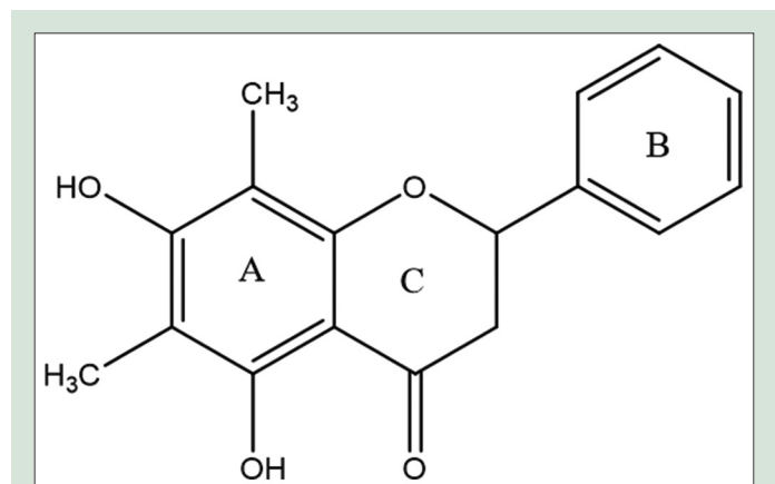
Figure 1: Structure of demethoxymatteucinol from Syzygium aqueum
