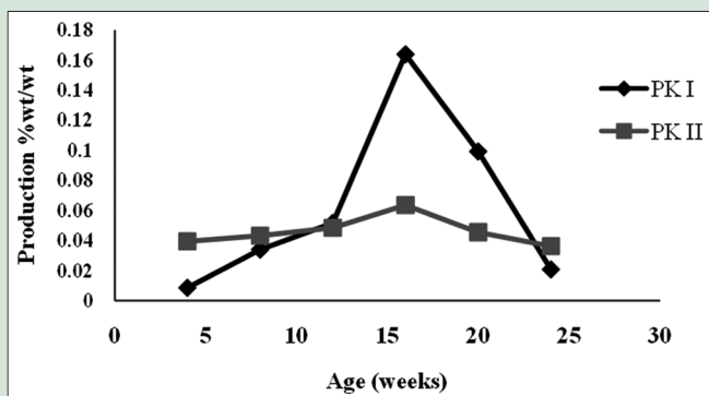
Figure 4: Production kinetics of Picoside-I and Picoside-II
