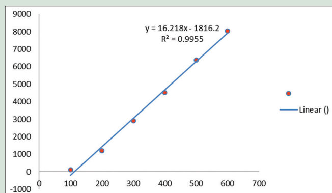
Figure 7: Calibration plot for quercetin standard
