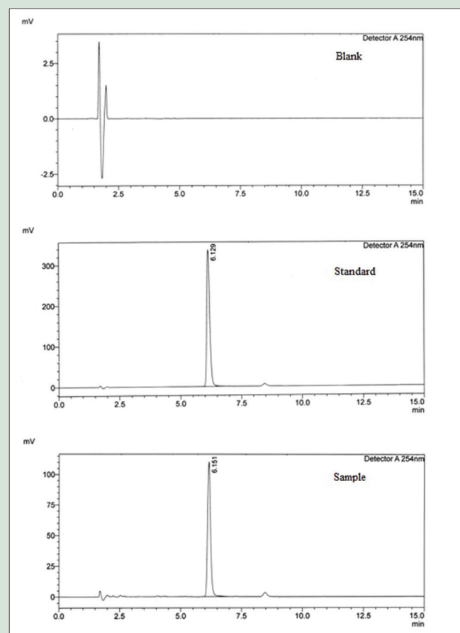
Figure 1: High-performance liquid chromatography chromatograms of blank, standard, and sample. The retention time of mangiferin standard and sample peak were found at 6.129 and 6.151, respectively. The theoretical plates and tailing factor of standard peak are 11763 and 1.307 were observed
