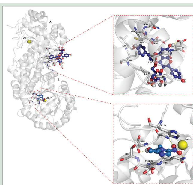
Figure 3: Inhibition sites over G/FBPA to metronidazole and tiliroside (left panel). Close contact of the binding modes of metronidazole (lower right panel) in short distance to Zn 2+ atom and tiliroside (upper right panel). H bonds are showed in red dashes. G = Gly, N = Asn; L = Leu, P = Pro, H = His, V = Val, S = Ser, E = Glu, C = Cys, D = Asp, I = Ile, and K = Lys
