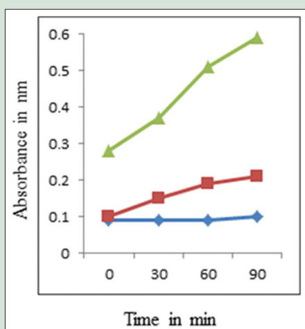
Figure 4: Effects of the Mentha piperita essential oil on the 260 nm absorbing material release of Fusarium sporotrichioides ([▲]: control; [■]: Minimum inhibitory concentration; [◆]: Minimum fungicidal concentration)
