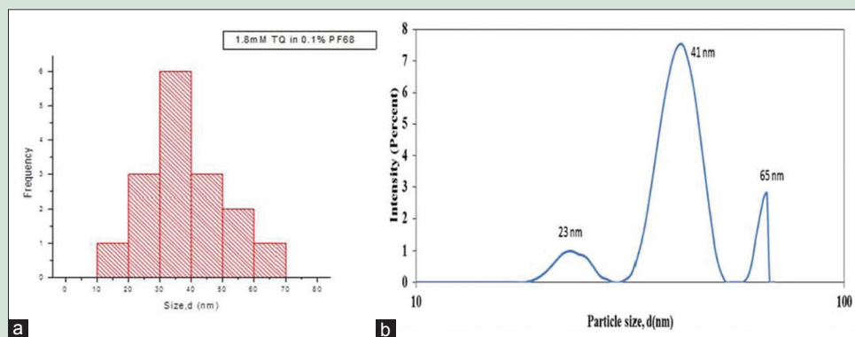
Figure 7: (a) Particle size distribution for 1.8 mM thymoquinone loaded 0.1% PF68 ( 37.74 \pm 12.94 ) nm (b) Average hydrodynamic size for 1.8 mM thymoquinone loaded 0.1% PF68
