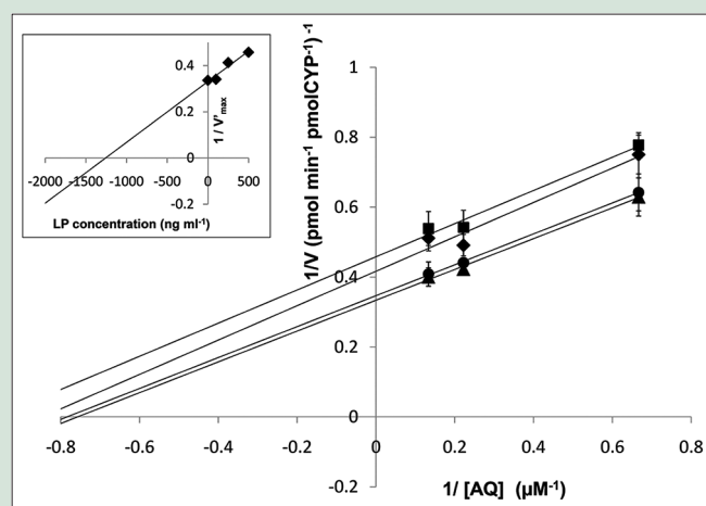
Figure 2: Primary Lineweaver-Burk plot and secondary plot (inset, 1/V' vs. inhibitor concentration) for the inhibition of cytochrome P450 2C8-mediated amodiaquine N-desethylation by Labisia pumila extract. Reactions were performed in the presence of amodiaquine at three different concentrations (1.5 \mu M, 4.5 \mu M, and 7.5 \mu M) at 0 ng/ml (▲), 100 ng/ml (●), 250 ng/ml (◆), and 500 ng/ml (■) of the extract in the presence of cytochrome P450 2C8 recombinant protein (3 pmol/ml) and NADPH system in 100 mM phosphate buffer (pH 7.4), at a final volume of 1 ml at 37°C for 20 min. Each point represents the mean of separate experiments performed in triplicates
