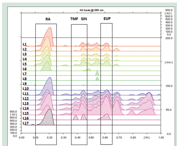
Figure 3: High-performance thin-layer chromatography chromatogram for Orthosiphon stamineus extracts with four identified compound; 3'-hydroxy-5,6,7,4'-tetramethoxyflavone, sinensitin, eupatorin and rosmarinic acid legend: L1: SBEW L2: CJEW L3: SEW L4: KBEW L5: BKEW L6: SBW L7: CJW L8: SW L9: KBW L10: BKW L11: SBE L12: CJE L13: SE L14: KBE L15: BKE L16: Mix standards; 3'-hydroxy-5,6,7,4'-tetramethoxyflavone, sinensitin and eupatorin L17: Rosmarinic acid
