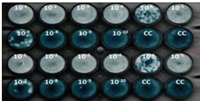
Figure 1: Plaque assay for Japanese encephalitis virus (JEV) vero cell line the titration of JEV was performed in vero cell line by plaque assay. The titre of the JEV stock was be 50 \times 10^7 PFU/ml
