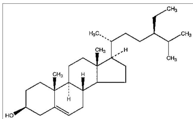
Figure 3: Structure of isolated Compound 3 (β-sitosterol)
