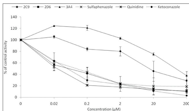
Figure 2: Inhibitory effect of mitragynine, sulfaphenazole, quinidine and ketoconazole on human cytochrome P450 2C9, 2D6 and 3A4 using recombinant enzymes. Each data represents the value of mean \pm SEM for three determinations (n=3) of two independent experiments
