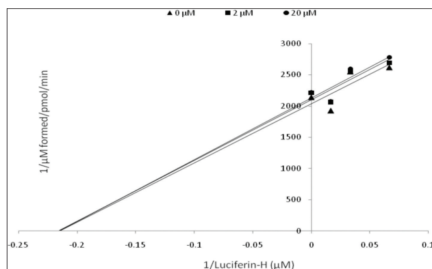
Figure 3: Lineweaver-Burk plot of the inhibitory effect of mitragynine on CYP2C9 activity. Each data represents the value of three determinations (n=3)
