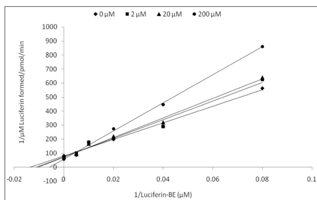
Figure 7: Lineweaver-Burk plot of inhibitory effect of mitragynine on CYP3A4 activity
