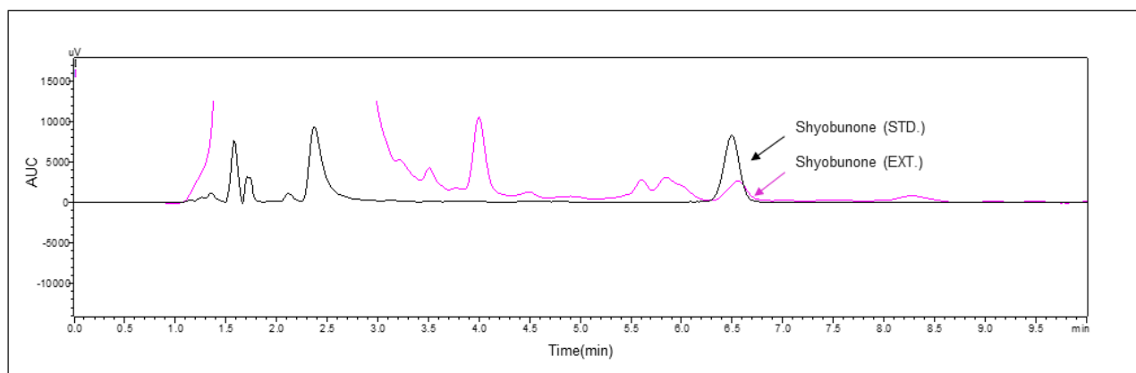
Figure 3: Overlaid chromatograms of 50 µg/mL standard solution of shyobunone and 1000 µg/mL solution of Acorus calamus ethanolic extract sample at 210 nm by using mobile phase 0.05% Ortho Phosphoric Acid (OPA) in water, acetonitrile and methanol (15:40:45). Abbreviations: STD: Standard marker compound; EXT: Extract sample.
