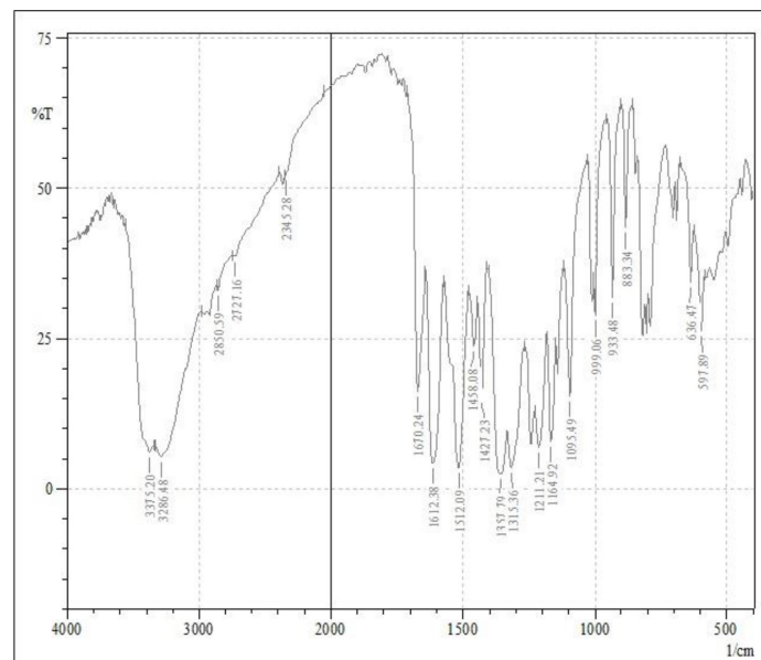
Figure 4: FT-IR of compound IO1.
