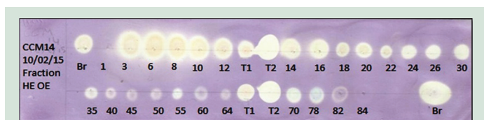
Figure 2: Image of the silica plate with the essential oil fractions of Origanum elongatum after 15 min reaction with DPPH. DPPH at 6 \cdot 10^{-5} M. Br: Crude essential oil, 1-84: Selected fractions. T1: \delta -tocopherol; T2: Ascorbic acid. DPPH: 2,2-diphenyl-1-picrylhydrazyl
