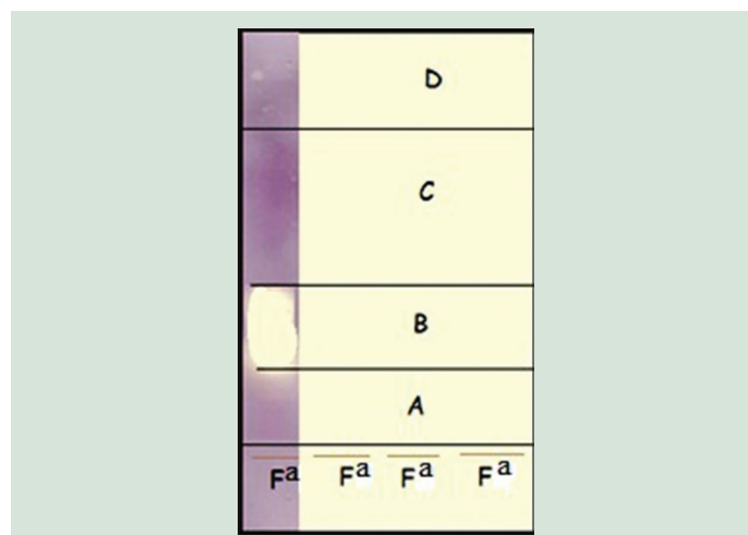
Figure 5: Representation of the preparative TLC plate and the various fractions to be recovered (A, B, C, and D). TLC: Thin-layer chromatography
