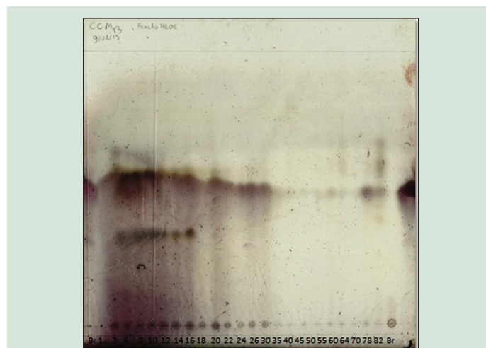
Figure 3: Chromatogram of the different fractions from the essential oil of Origanum elongatum after migration and visualization by sulfuric acid. Br: Crude essential oil, 1, 3, 6; 82: Fractions; Eluent: (hexane/diethyl ether/ethyl acetate, 60/35/5, v/v/v)
