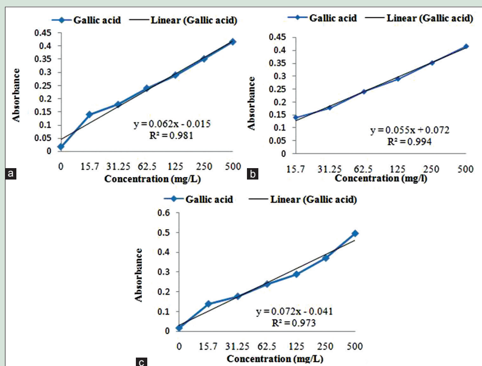
Figure 2: Determination of total phenolic contents of (a) Bougainvillea glabra (b) Licuala grandis and (c) Anthurium crystallinum with the help of gallic acid standard calibration curve
