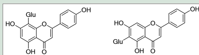
Figure 2: Chemical structures of A: Vitexin and B: Isovitexin. Glu: Glucose
