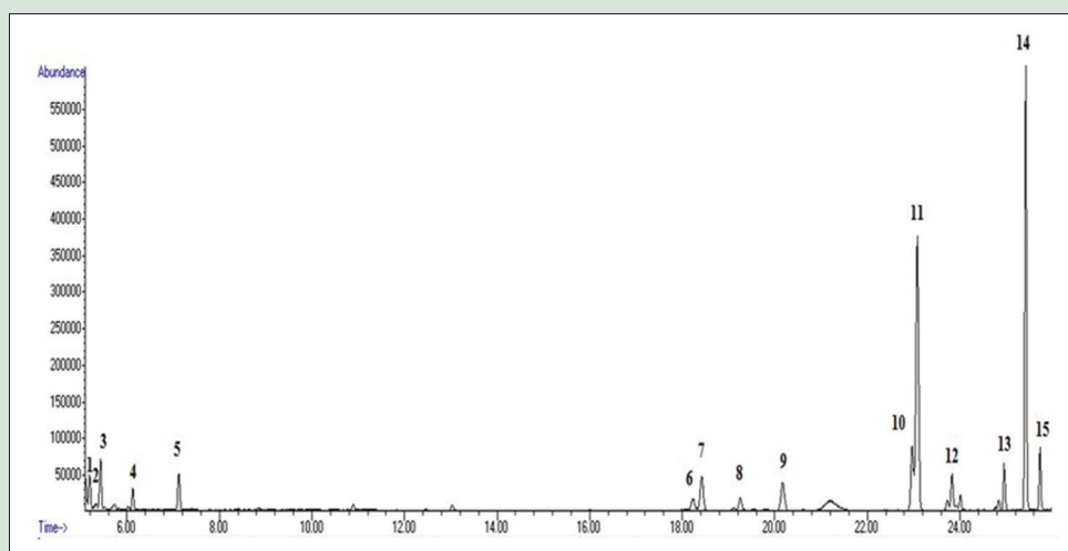
Figure 1: Chromatogram of total ions obtained by gas chromatography coupled to mass spectrometry of Hymenaea stigonocarpa resin. Numbered according to table 01
