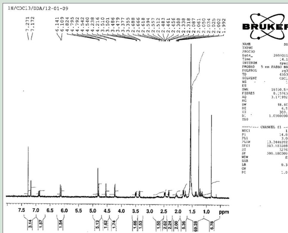
Figure 4: 1 H-NMR Spectral analysis of 14-deoxy-11, 12-didehydroandrographolide
