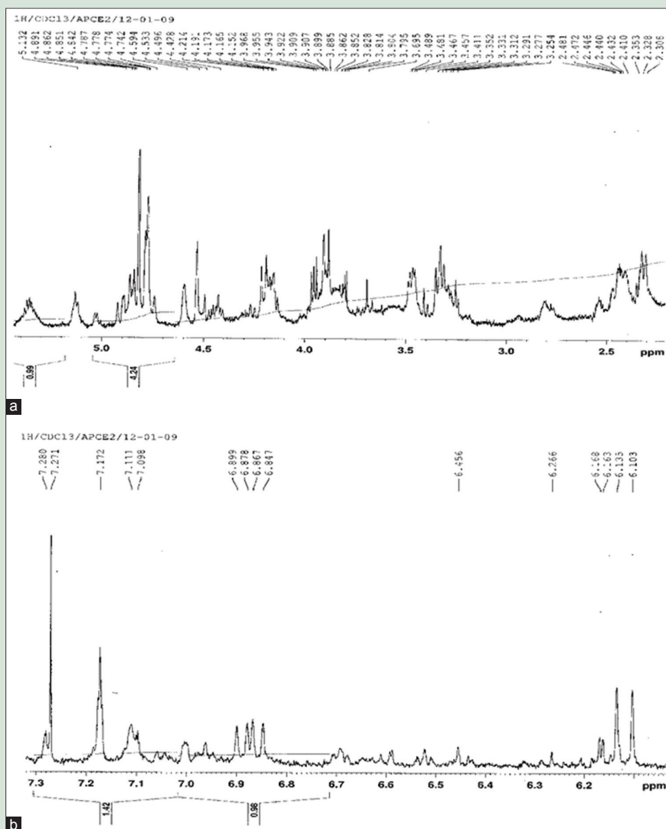
Figure 6: (a and b) 1 H-NMR Spectral analysis of Andrographis paniculata chloroform extract
