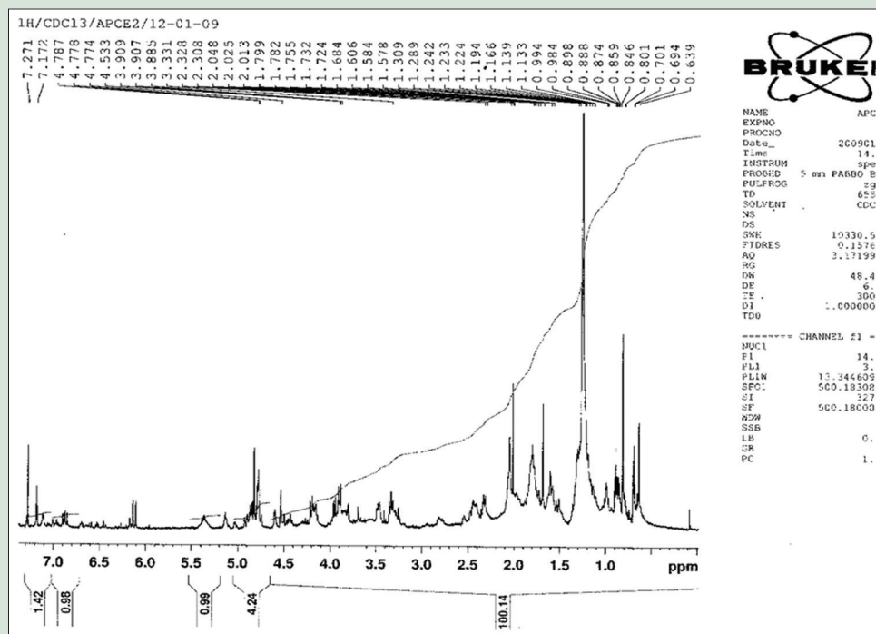
Figure 5: 1 H-NMR Spectral analysis of Andrographis paniculata chloroform extract
