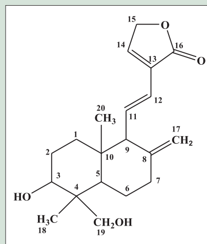
Figure 2: Chemical structure of DDA. Molecular formula: (C_{20}H_{28}O_4) . Molecular weight: 332.44 g
