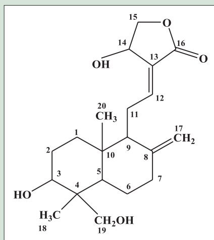
Figure 1: Chemical structure of Andrographolide. Molecular formula: C_{20}H_{30}O_5 . Molecular weight: 350.46 g
