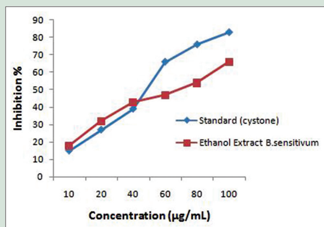
Figure 2: Nucleation assay
