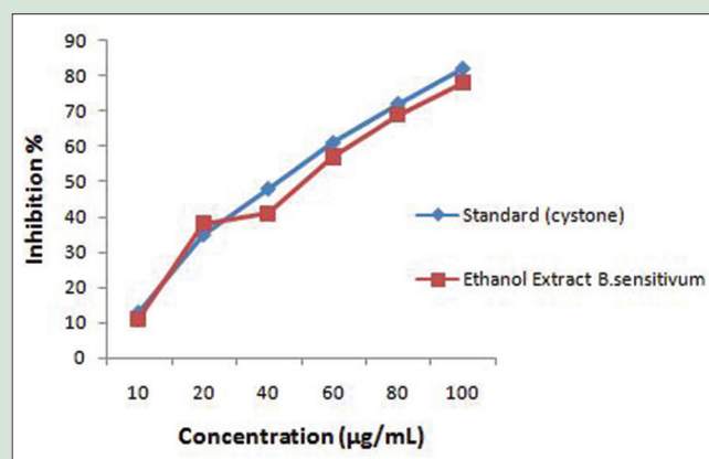
Figure 3: Aggregation assay
