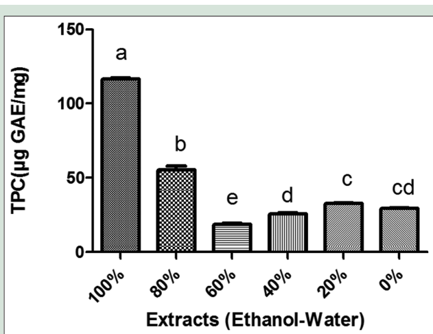
Figure 1: Total phenolic content of extracts with different solvent ratio (ethanol-water). Values are mean \pm standard deviation of triplicate analyses. Values followed by different letter are significantly different ( P < 0.05 )
