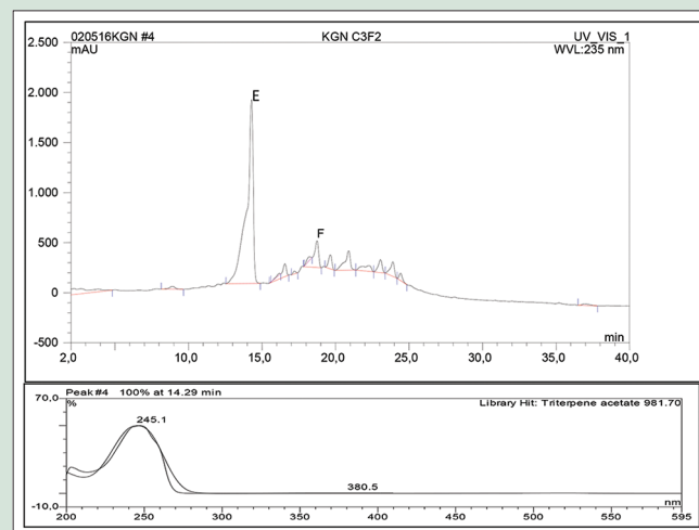
Figure 3: High-pressure liquid chromatography chromatogram of ethyl acetate fraction (AC3) and ultraviolet chromatogram of triterpene acetate. E: Peak 4
