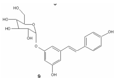
9: Trans-resveratrol-3-O-glucoside
